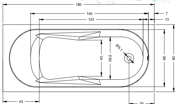
WANNA LAZY BC41 180x80 cm
