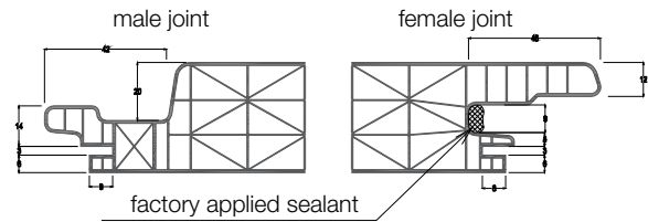
Joint Detail
