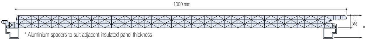
Aluminium Spacer Profiles
